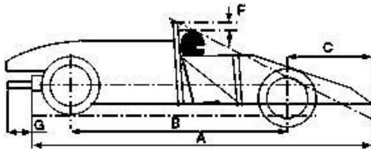
SAFETY ROLL-OVER BAR, WITHOUT STEERING BULKHEAD ROLL-OVER BAR
